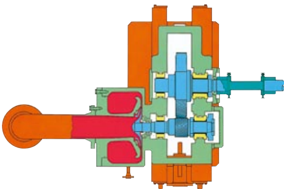
POB-GH Compressor
