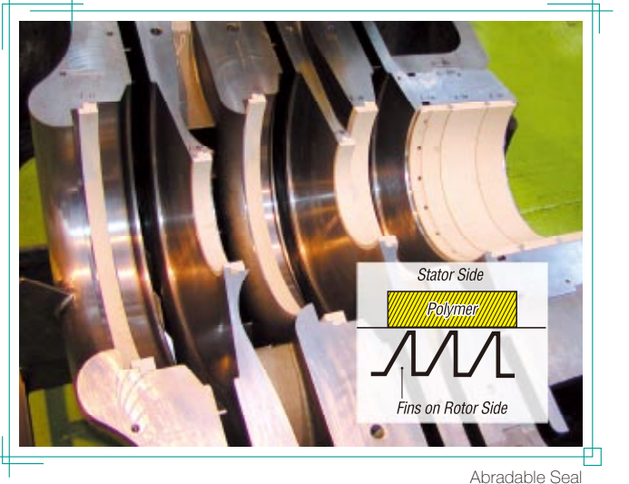
Abradable Seal
