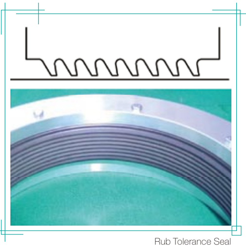
Rub Tolerance Seal
