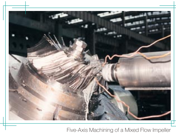
Five-Axis Machining of a Mixed Flow Impeller
